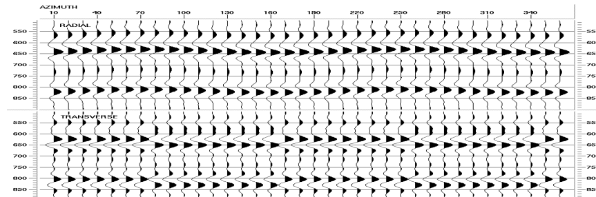
Figure 4: The same as Figure 2 except that each trace is scaled individually. Notice the abrupt polarity change in the transverse wavelet at the S1 and S2 azimuths, and the 90^\circ phase difference between the radial and transverse wavelets.
