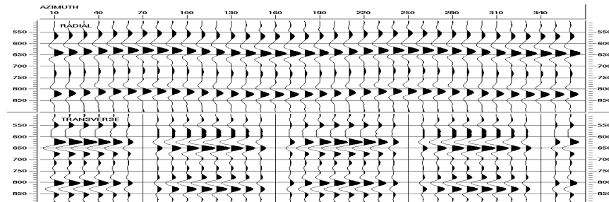
Figure 3: Limited-azimuth stacks for a single anisotropic layer. The S1 azimuth is 70^\circ and S2 arrives 14 ms after S1.
