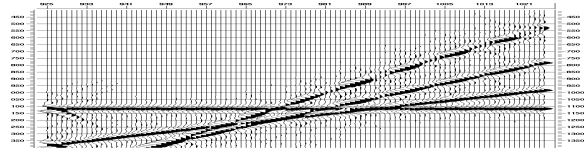
Fig. 15 Offset continuation of a pseudo-common-offset section.
