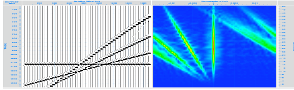
Fig. 4 An aliased true common-offset section.
